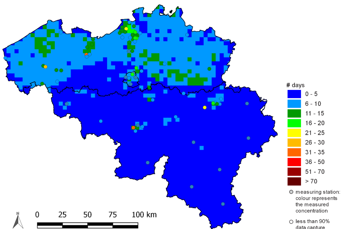
Number of days with daily mean PM 10 > 50 µg/m 3 (Belgium, 2018)
