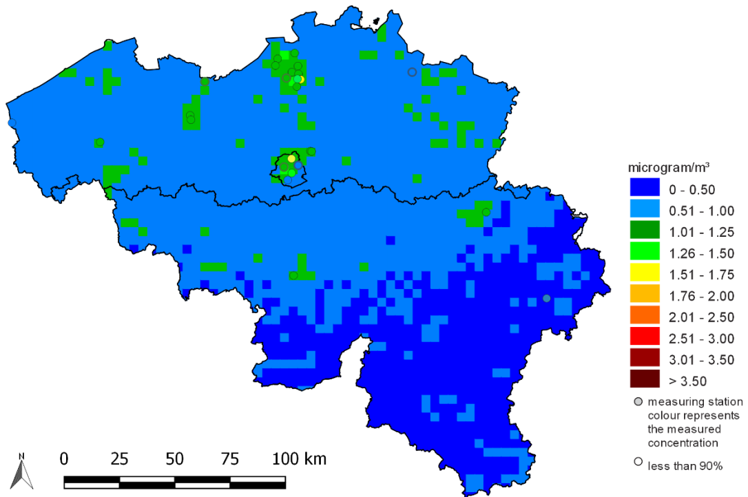
Annual mean BC concentration (Belgium, 2018)
