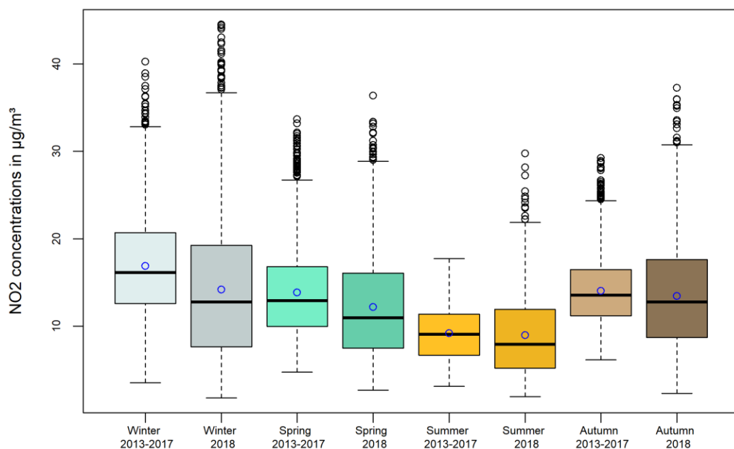
Spatial average NO 2 concentrations per season
