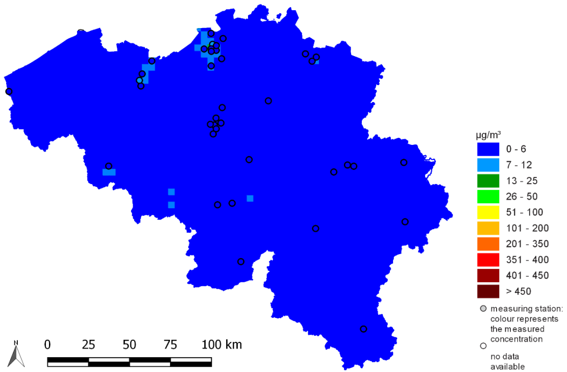
25th highest hourly mean SO 2 (Belgium, 2018)
