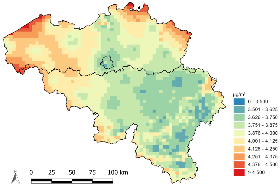
Error on PM2.5 annual mean (Belgium, 2016)
