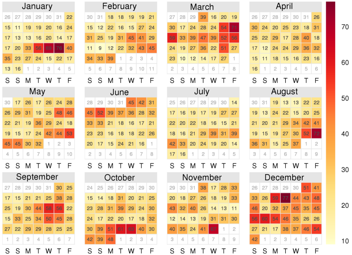
Mean daily PM 10 concentrations in 2016
