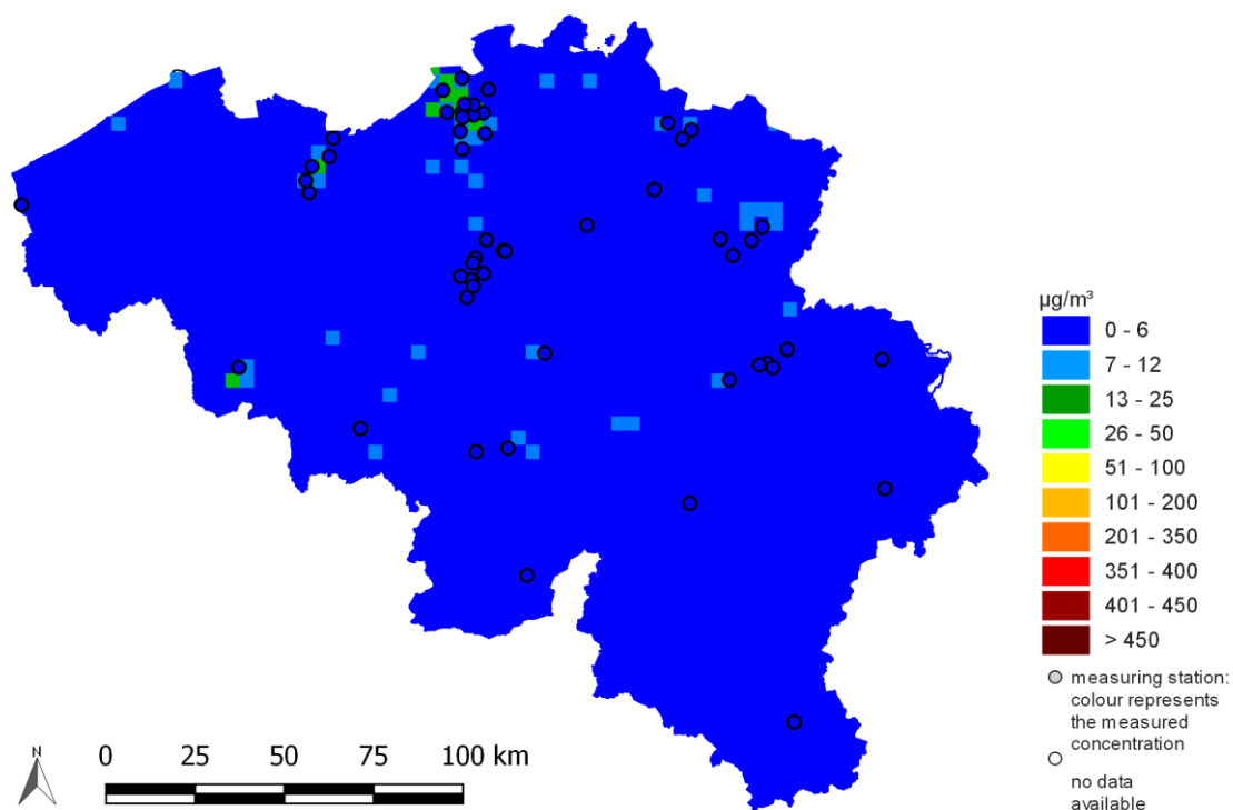
25th highest hourly mean SO 2 (Belgium, 2016)
