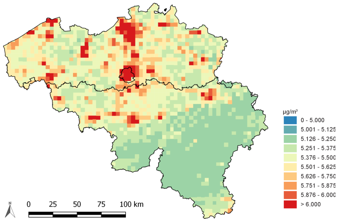
NO 2 annual mean absolute error (Belgium, 2016)
