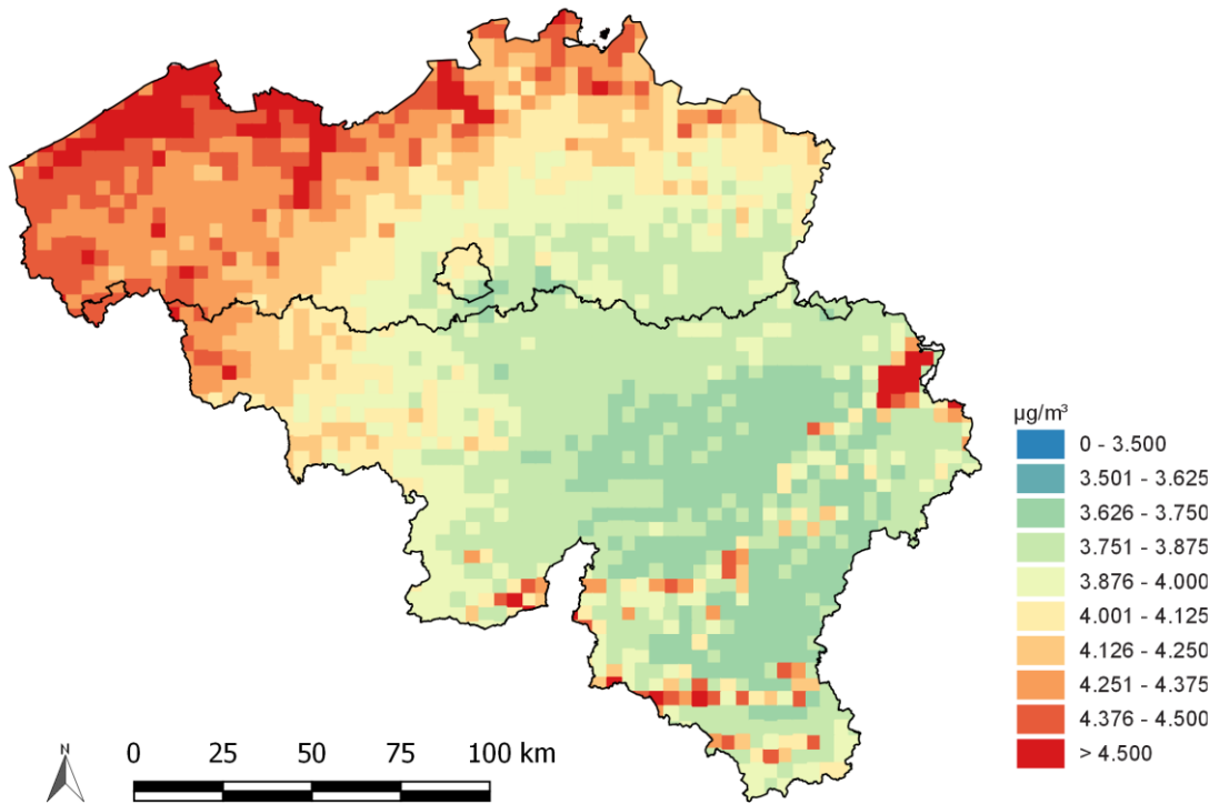
Error on PM10 annual mean (Belgium, 2016)
