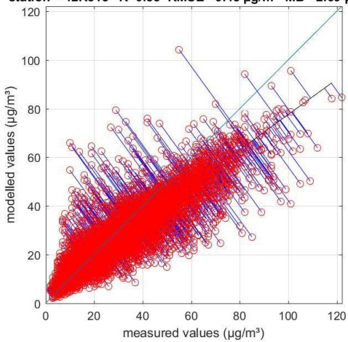
station = '42R815' R=0.88 RMSE =9.48 \mu\text{g}/\text{m}^3 MB=-2.69 \mu\text{g}/\text{m}^3
