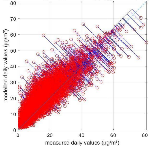
station =RMHA06 R=0.87 RMSE =6.84 \mu\text{g}/\text{m}^3 MB=3.65 \mu\text{g}/\text{m}^3
