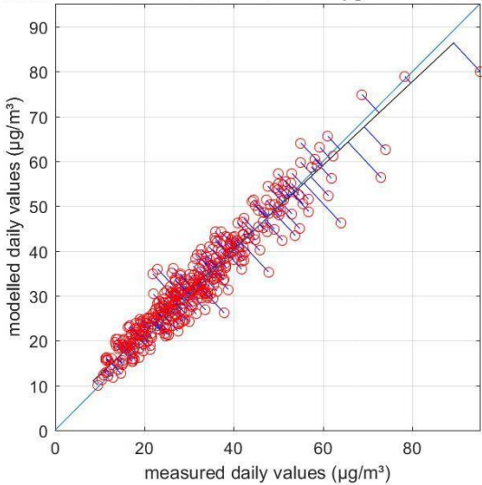
station = '42R803' R=0.95 RMSE =4.21 \mu\text{g}/\text{m}^3 MB=0.96 \mu\text{g}/\text{m}^3
