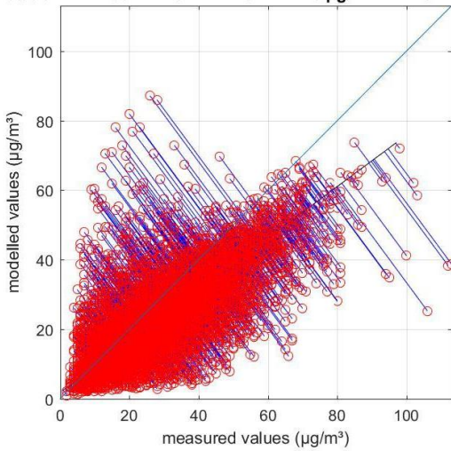
station='42R831' R=0.71 RMSE =12.25 \mu\text{g}/\text{m}^3 MB=-5.41 \mu\text{g}/\text{m}^3
