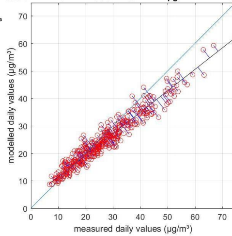
station = '42R815' R=0.96 RMSE =5.38 \mu\text{g}/\text{m}^3 MB=-2.76 \mu\text{g}/\text{m}^3
