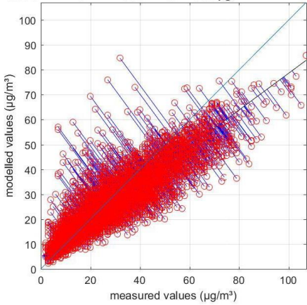
station = '42R815' R=0.88 RMSE =9.48 \mu\text{g}/\text{m}^3 MB=-2.69 \mu\text{g}/\text{m}^3
