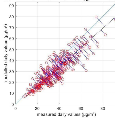
station='44R702' R=0.87 RMSE =9.31 \mu\text{g}/\text{m}^3 MB=-5.84 \mu\text{g}/\text{m}^3
