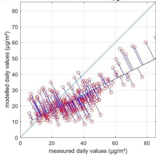
station =RMNA12 R=0.68 RMSE =14.66 \mu\text{g}/\text{m}^3 MB=-9.21 \mu\text{g}/\text{m}^3
