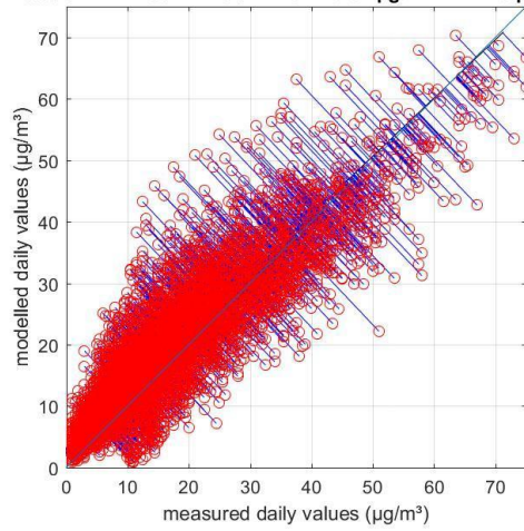
station =RMNA12 R=0.59 RMSE =18.6 \mu\text{g}/\text{m}^3 MB=-9.22 \mu\text{g}/\text{m}^3
