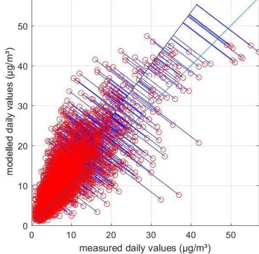
station =RMBU01 R=0.81 RMSE =4.89 \mu\text{g}/\text{m}^3 MB=2.92 \mu\text{g}/\text{m}^3
