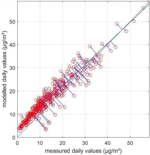
station =RMNA12 R=0.68 RMSE =14.66 \mu\text{g}/\text{m}^3 MB=-9.21 \mu\text{g}/\text{m}^3
