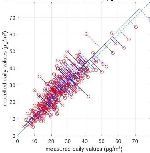
station =RMPT01 R=0.76 RMSE =4.87 \mu\text{g}/\text{m}^3 MB=-3.68 \mu\text{g}/\text{m}^3
