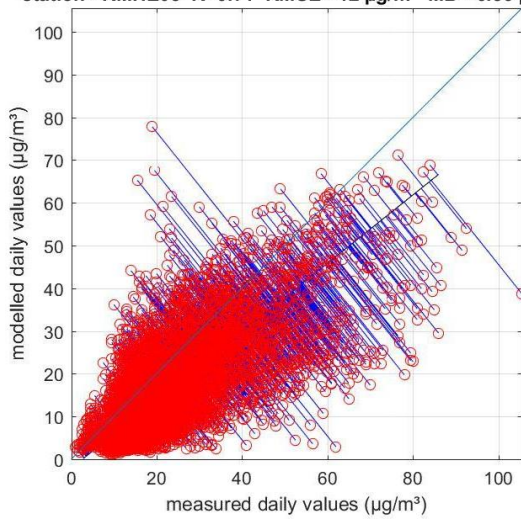
station =RMHE08 R=0.71 RMSE =12 \mu\text{g}/\text{m}^3 MB=-6.83 \mu\text{g}/\text{m}^3
