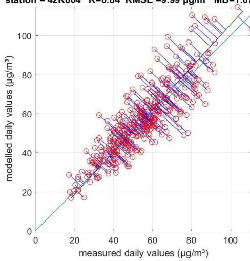
station='42R804' R=0.84 RMSE =9.99 \mu\text{g}/\text{m}^3 MB=1.67 \mu\text{g}/\text{m}^3
