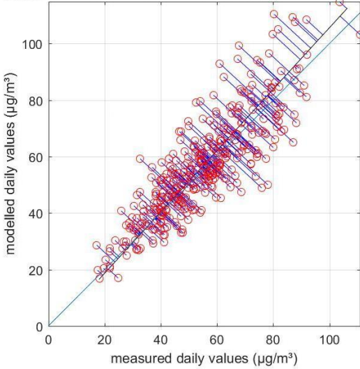
station = '42R804' R=0.84 RMSE =9.99 \mu\text{g}/\text{m}^3 MB=1.67 \mu\text{g}/\text{m}^3
