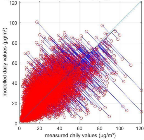
station =RMPT01 R=0.64 RMSE =6 \mu\text{g}/\text{m}^3 MB=-3.66 \mu\text{g}/\text{m}^3
