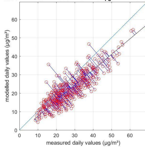
station='42R831' R=0.85 RMSE =7.81 \mu\text{g}/\text{m}^3 MB=-5.43 \mu\text{g}/\text{m}^3
