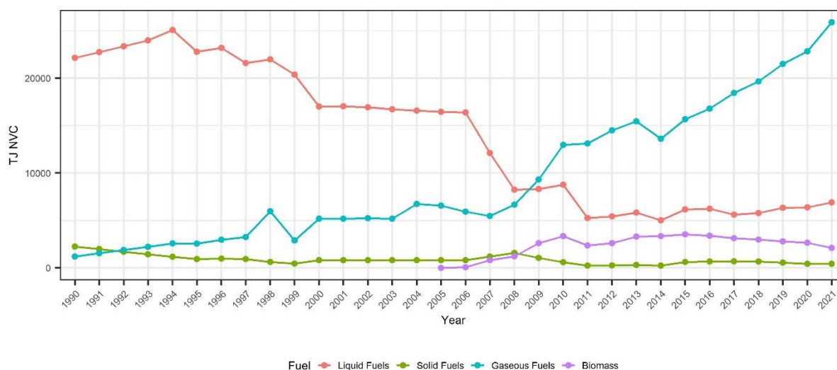
Figure 3-6 Trend of fuel consumption in the agricultural sector
