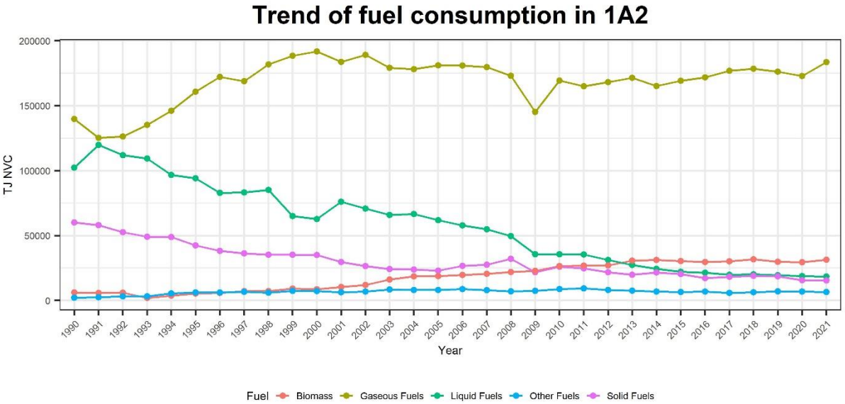
Figure 3-2 Trend of fuel consumption in the manufacturing Industries and construction.
