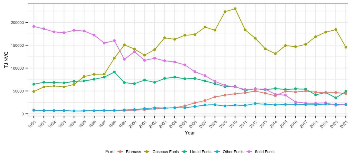
Figure 3-1 Trend of fuel consumption in the energy industries (1A1)
