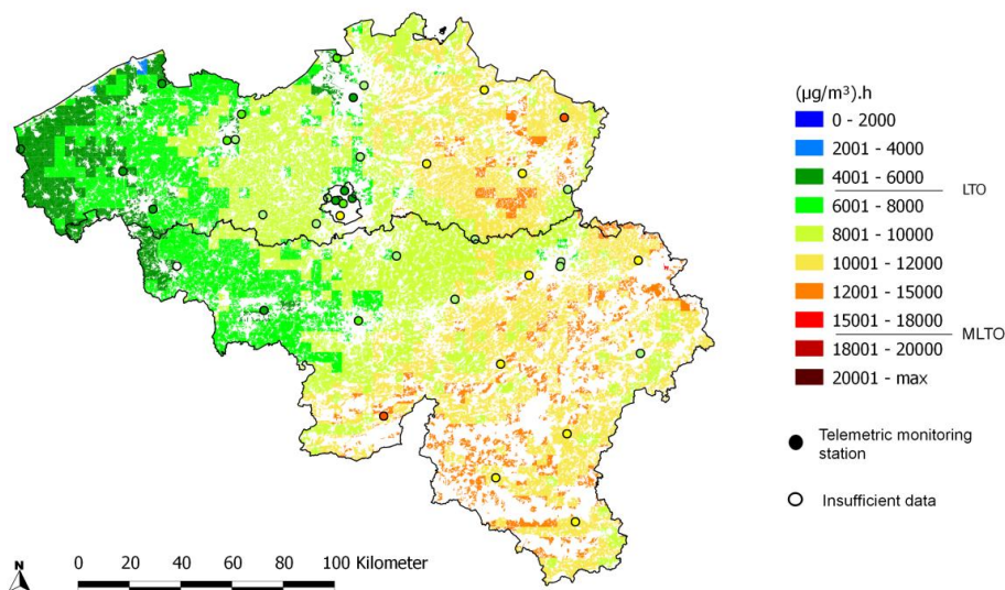
AOT40 vegetation (Belgium, 2008 - 2012)
